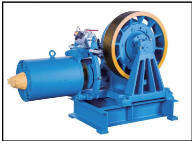
Gear Machine The elevator gear machine, also known as the elevator drive system or traction machine, is a mechanical system responsible for moving the elevator car vertically within the elevator shaft. Its primary function is to convert electrical energy into mechanical energy to lift and lower the elevator car.
